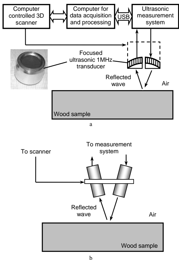
Fig. 2. Structure diagram of the experimental systems using focussed air – coupled 1 MHz dual element ultrasonic transducer (a) and a pair of planar 200 kHz transducers working in pitch – catch mode (b)
