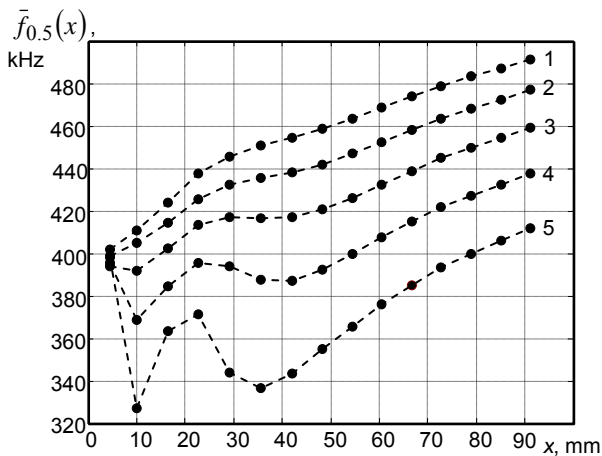
Fig.8. The equivalent frequencies of different half periods of the signal versus distance: 1-5 are the numbers of the half period
