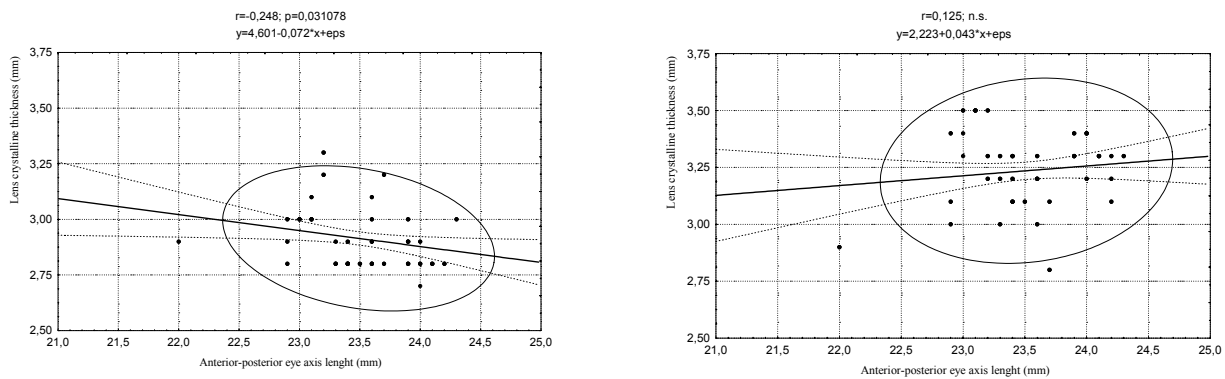
Fig. 3. The comparison of crystalline lens thickness and anterior-posterior eye axis length; static (to the left) and dynamic (to the right)
